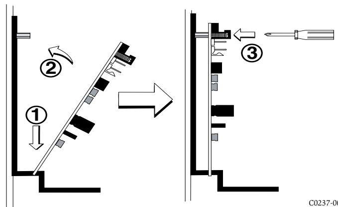
Figure 5: Installation of rear module only, method one
