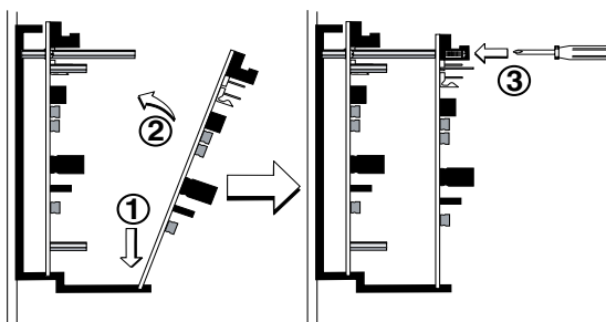
Figure 6b: Installation of CMF-300-6 module in front chassis position
