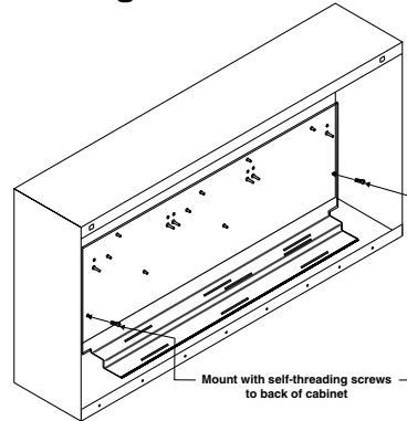
Figure 4: Mounting the CH-6 chassis
