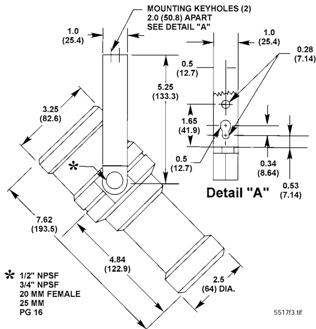
Figure 3 Dimensions in Inches (mm)
